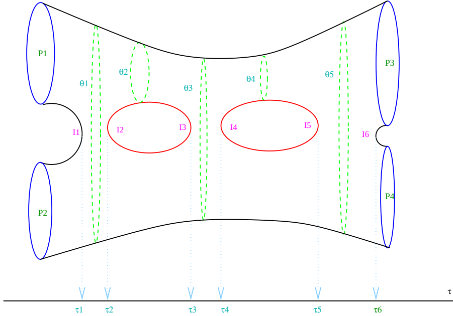
Figure 1: The string diagram of the spectral cover with interaction points I_i , i = 1..6 . The interaction times \tau_i and the angles \theta_i define the location of the interaction points. The external states correspond to the marked points P_i , i = 1..4
